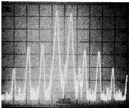
Fig. 3 — Spectral display of the TS-430S output during transmitter two-tone IMD test. Third-order products are 31 dB below PEP, and fifth-order products are 34 dB down. Vertical divisions are each 10 dB; horizontal divisions are each 1 kHz. The transceiver was being operated at rated input power on the 10-meter band.
