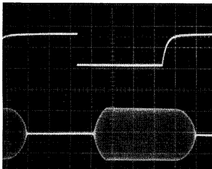
Fig. 4 — CW keying waveform of the TS-430S. The upper trace is the actual key closure; lower trace is the RF envelope. Each horizontal division is 5 ms. This RF waveform has good shaping.
