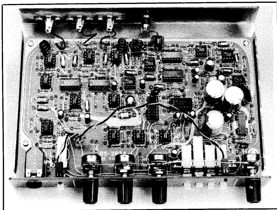
Fig. 5 — A peek inside the filter shows the large number of components used. The board layout is not too dense, however, and the board is easy to work on.
