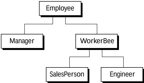
Figure 8.1 A simple object hierarchy
