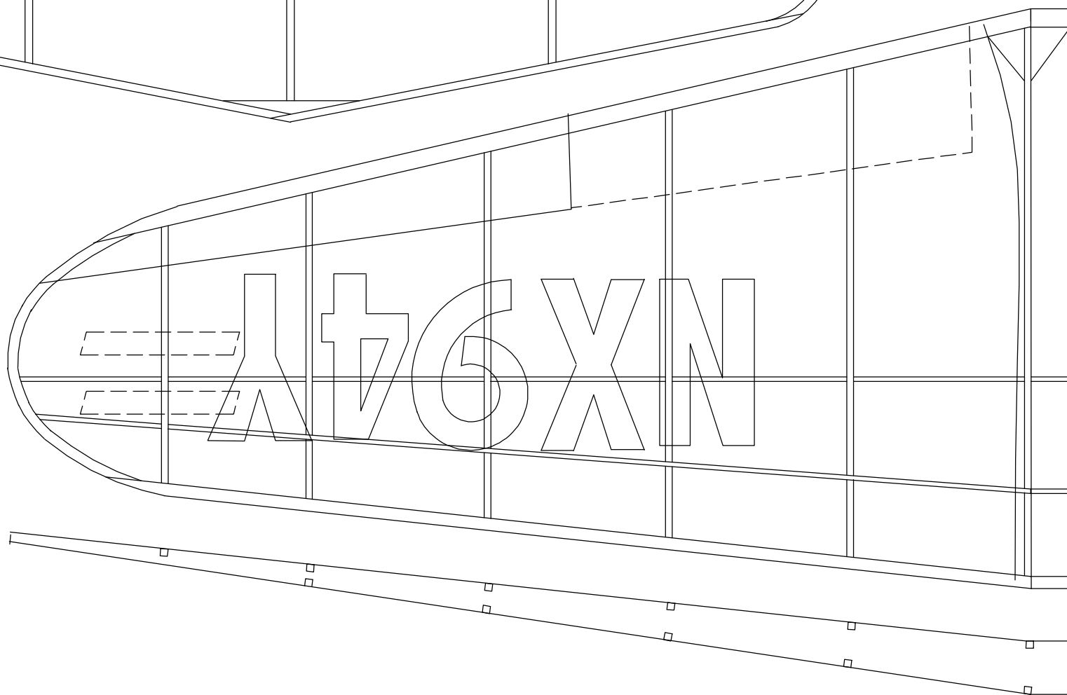
Removable Noseblock
