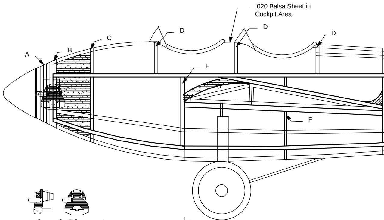
Bristol Cherub 32 HP Engine
