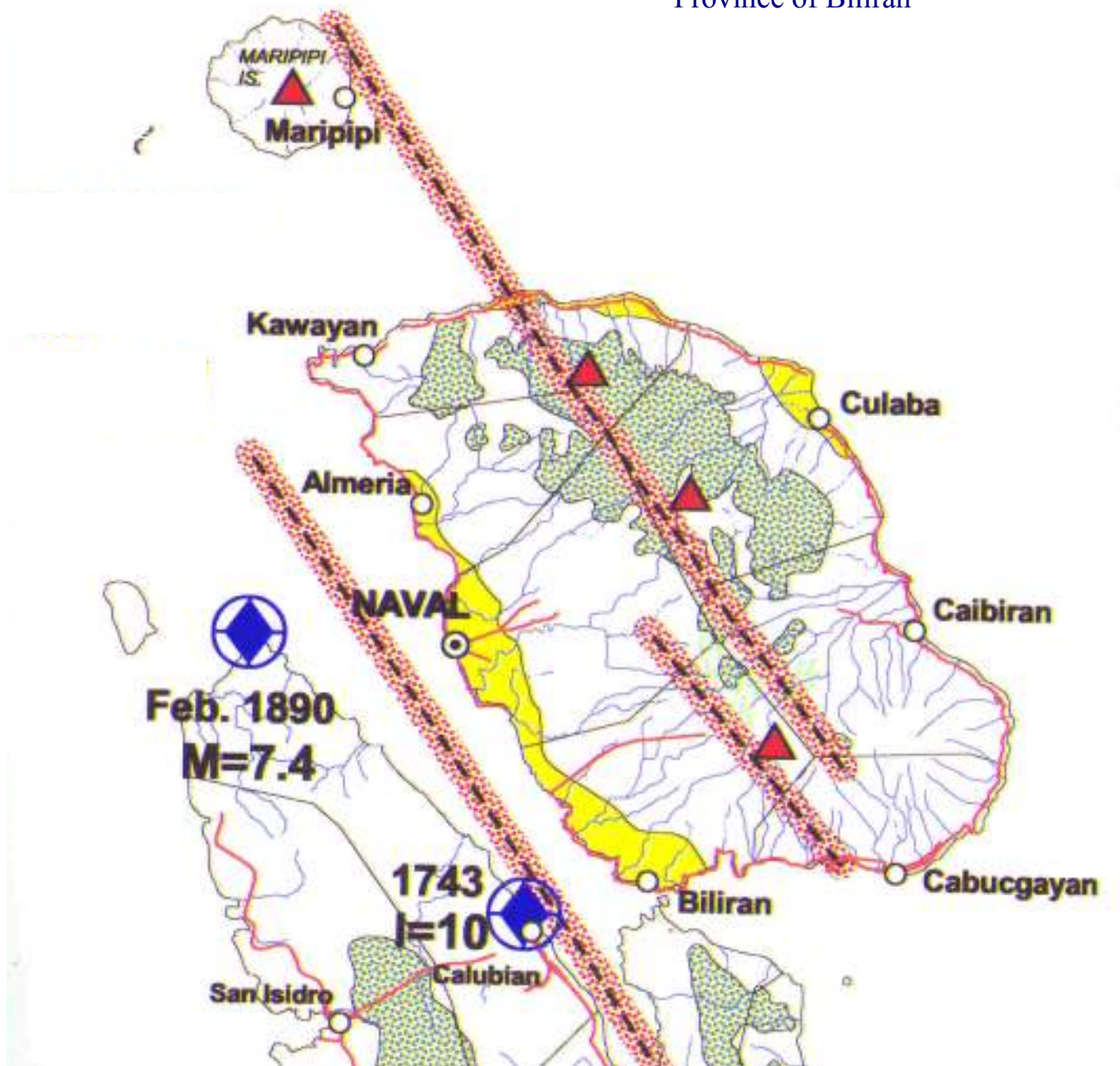
Figure B-19 GEO-HAZARD MAP Province of Biliran
