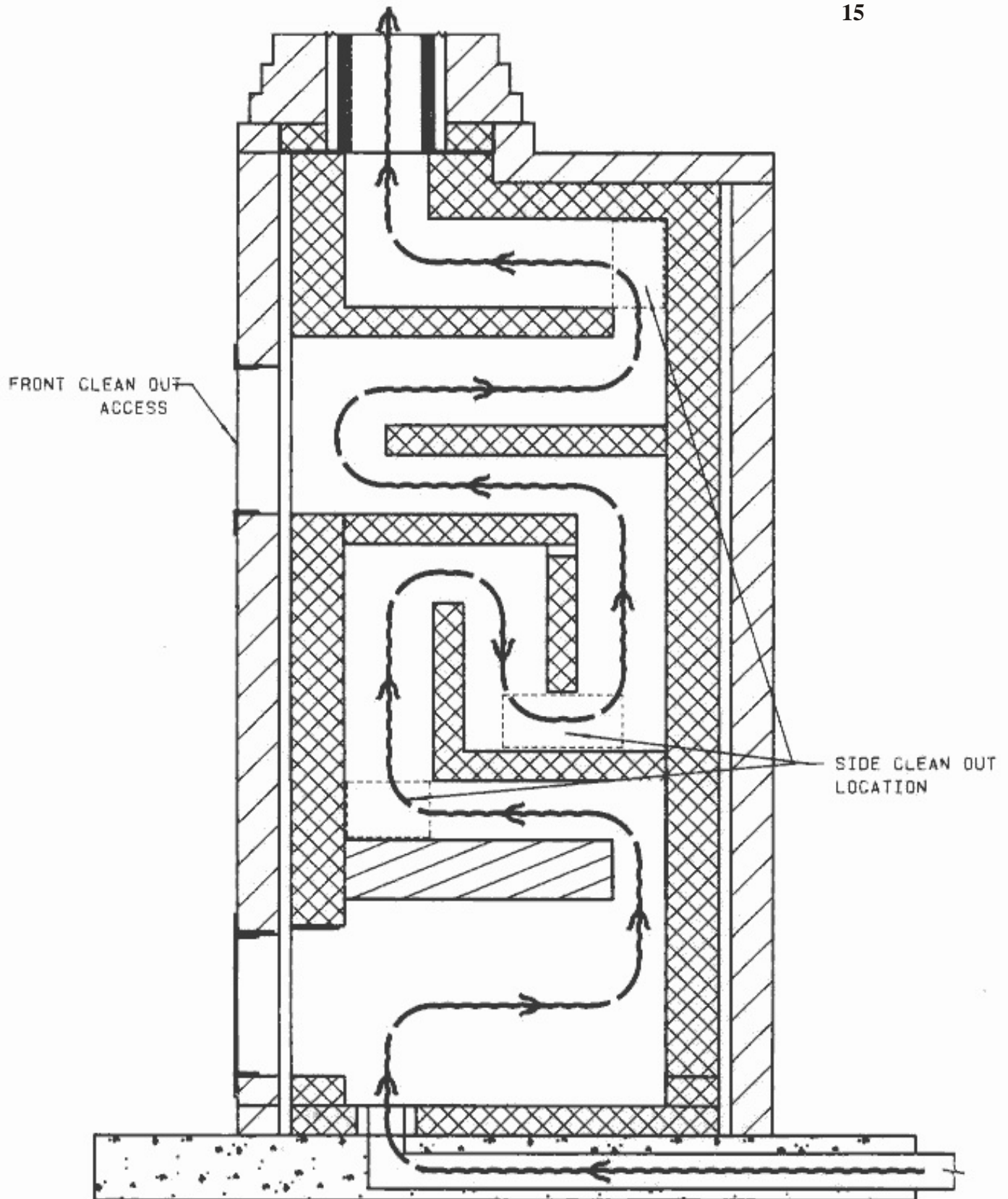
MASONRY STOVE WITHOUT OVEN VERTICAL FLUE RUN
