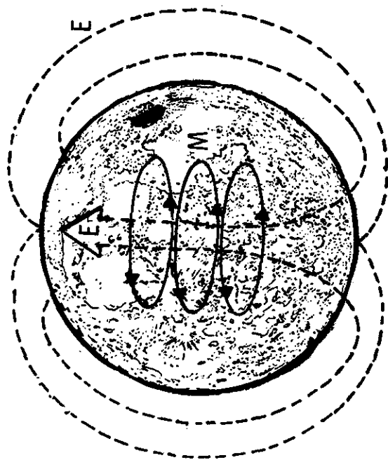
MAGNETIC FIELD OF MOON (M) GENERATED BY THE ELECTRIC FIELD E CARRIED IN THE SOLAR WIND
